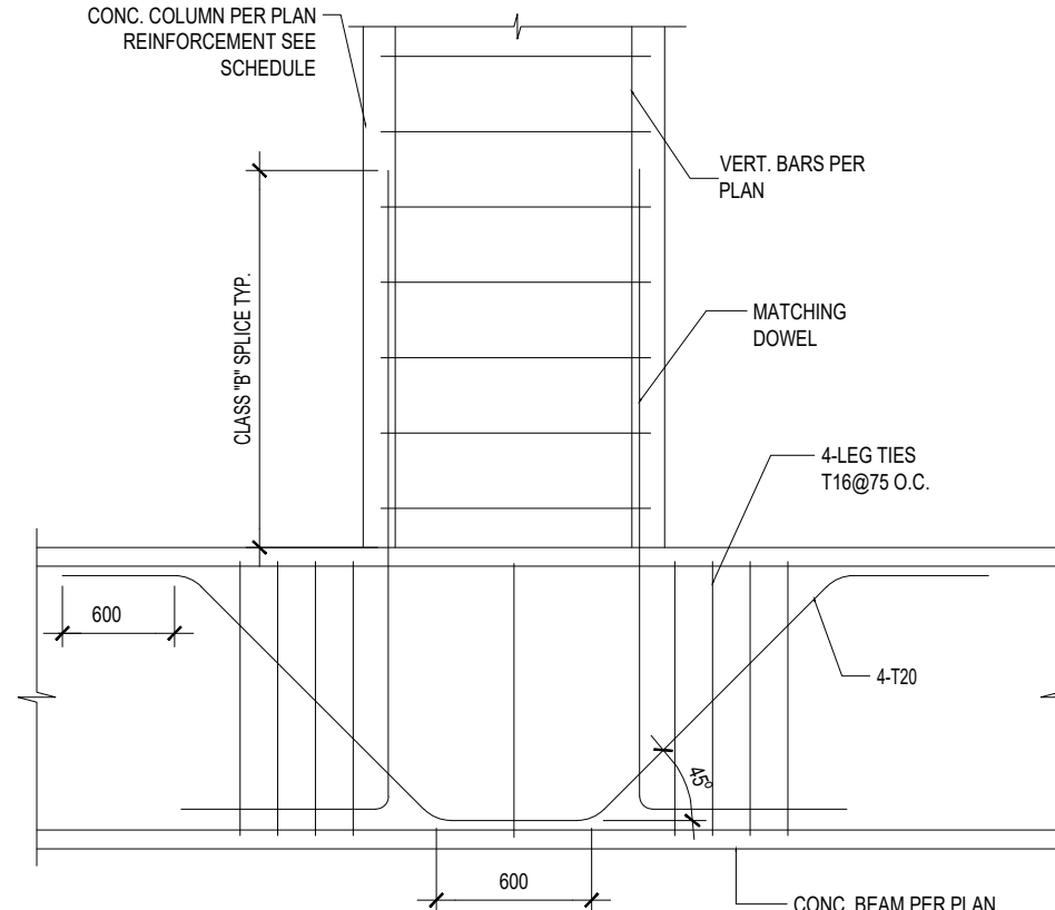
BEAM SUPPORTING COLUMN
