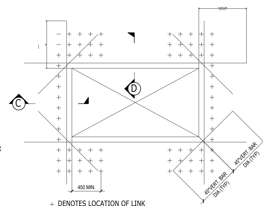
WALL OPENING GREATER THAN 450mm & LESS THAN 900mm
