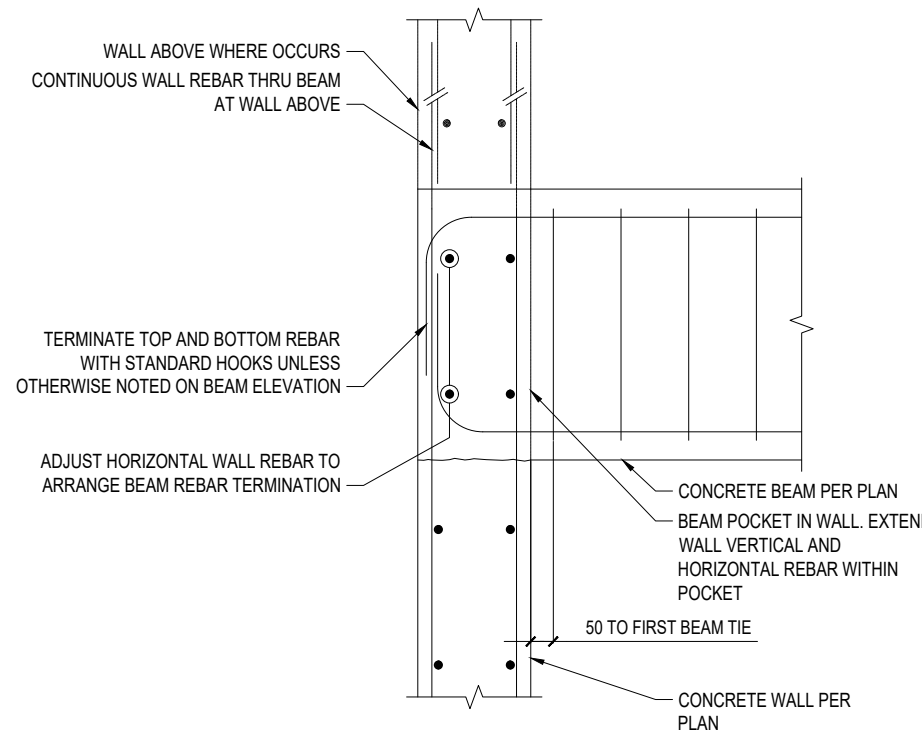
END SUPPORT
