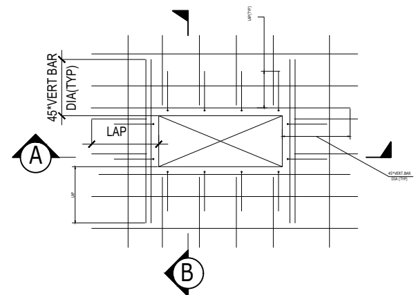
WALL OPENING GREATER THAN 150mm & LESS THAN 450mm
