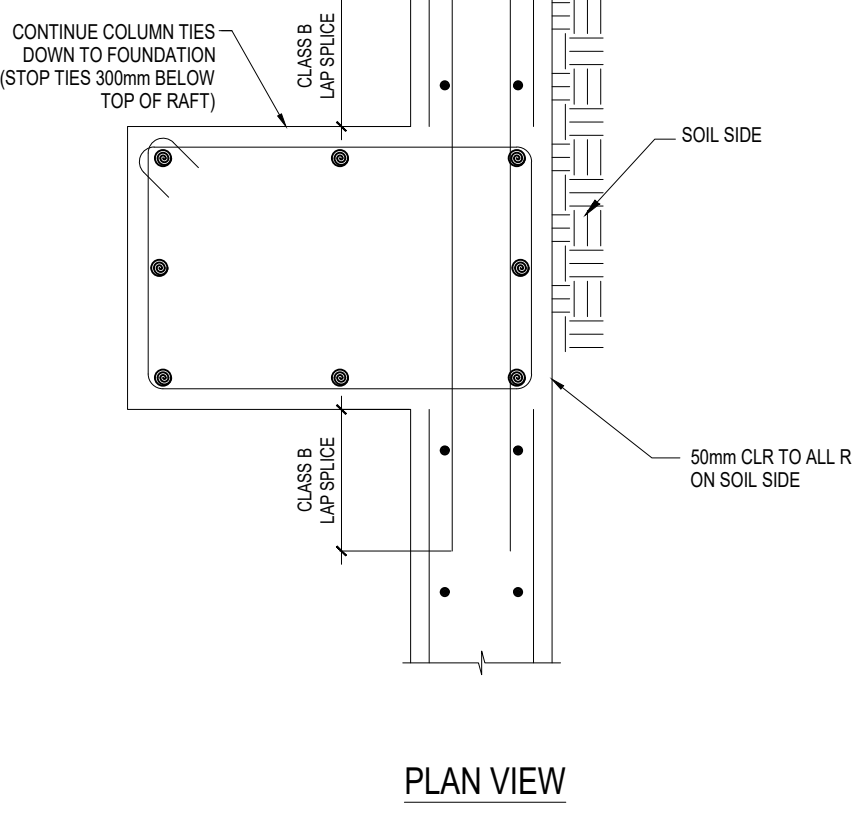
PERIMETER COLUMN AT BASEMENT WALL
