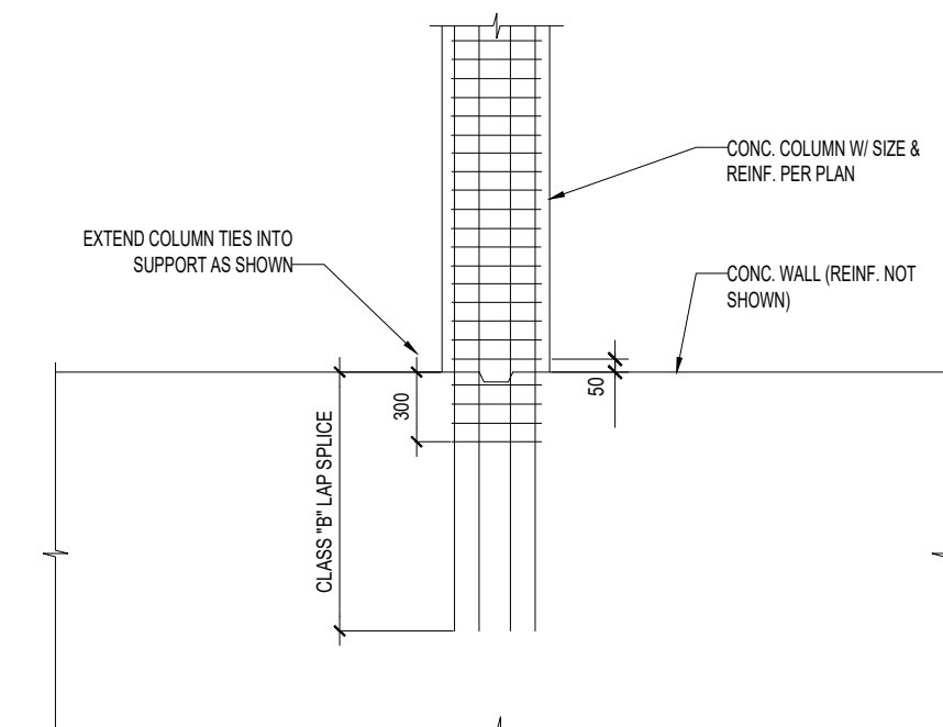
TYP. CONC. COLUMN ON WALL
