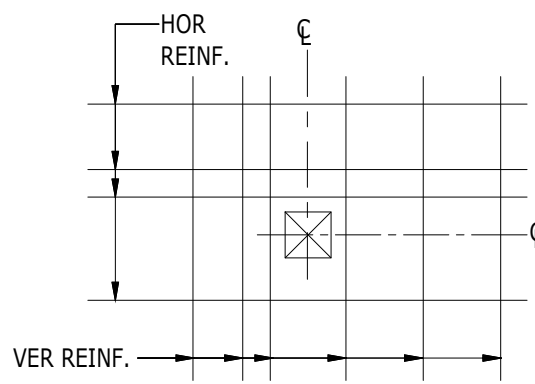
WALL OPENING LESS THAN 150mm
